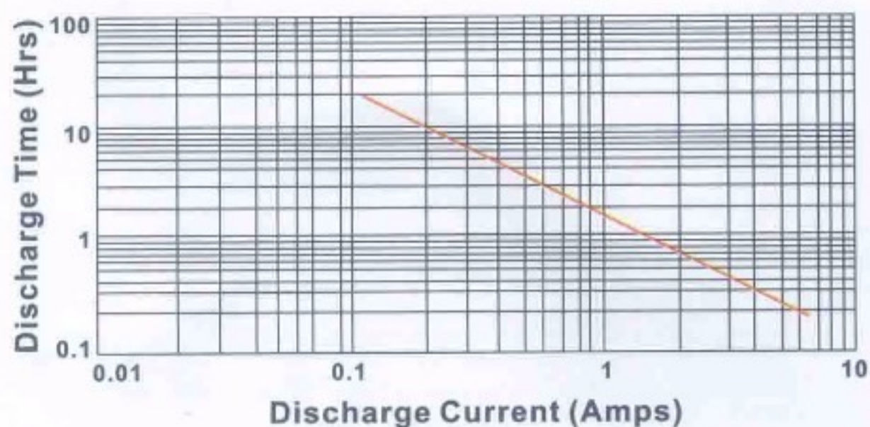
Discharge time Vs. Discharge current @ 77°F(25°C)
