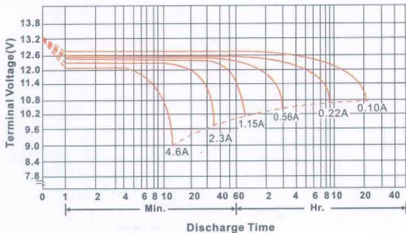
Discharge Characteristics @ 77°F(25°C)
