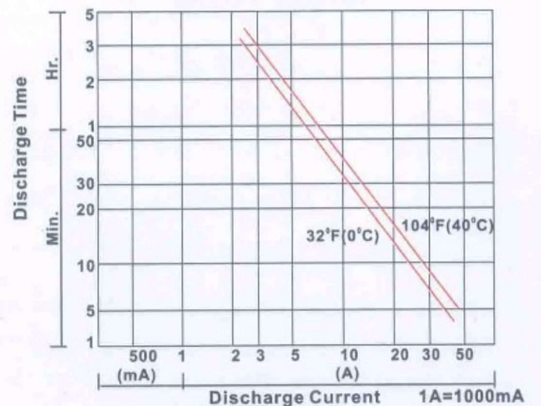
Discharge Time Vs. Discharge current
