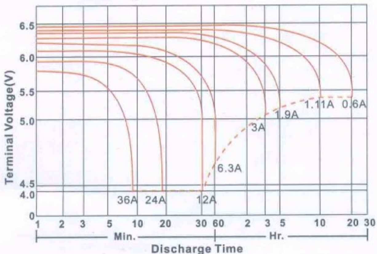
Discharge Characteristics @ 77°F(25°C)
